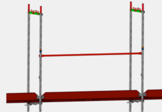
Figure 23: Recommended anchorage points on the vertical frame
