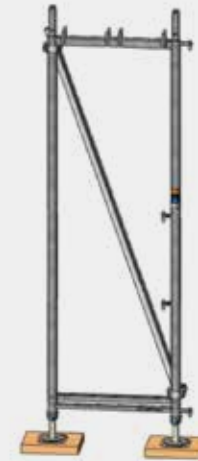
Figure 14: Vertical frame with transverse diagonal
