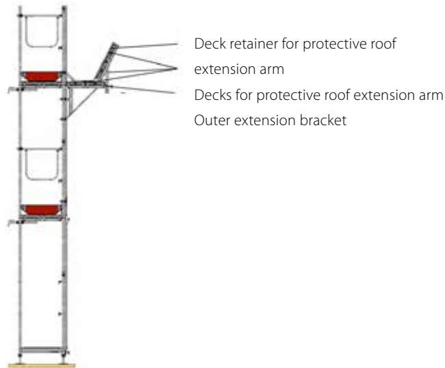
Figure 58: Protective roof
