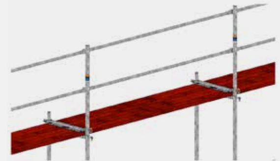
Fig. 45: Upper finish section with guardrail posts and deck retainers
