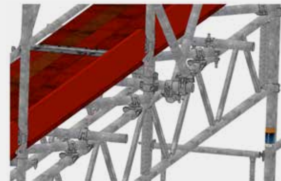
Figure 57: Connection of diagonal braces with standard couplers
