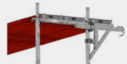
Figure 37: Short tie bar, version with inner extension brackets
