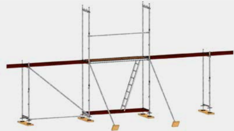
Figure 20: Example of a temporary anti-topple system for the first scaffolding level
