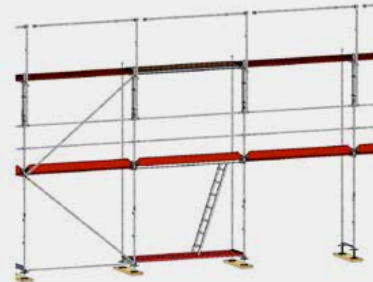
Figure 29: Fitting of additional mounting safety guardrail units
