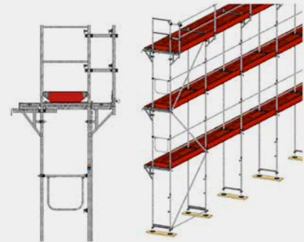
Figure 51: Scaffold with outer and inner single-deck extension brackets
