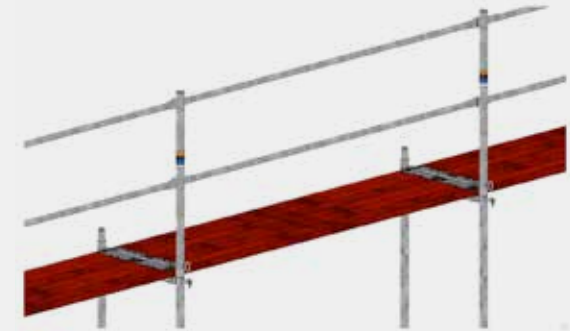
Fig. 44: Upper finish section with guardrail posts with transoms
