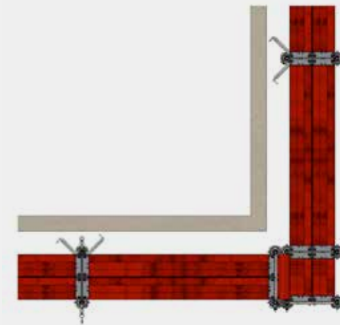
Figure 42: Anchorage at corners, structure with three vertical frames
