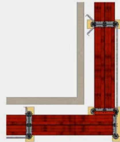
Figure 41: Anchorage at corners, structure with two vertical frames
