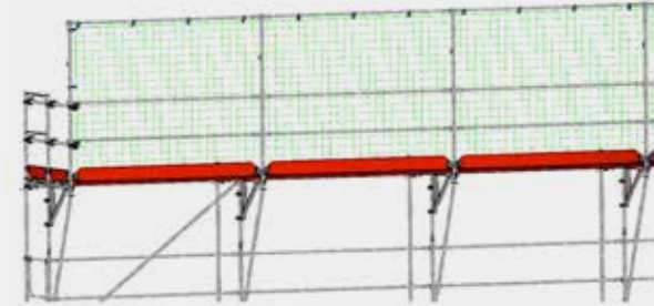
Figure 61: Protective wall on extension brackets
