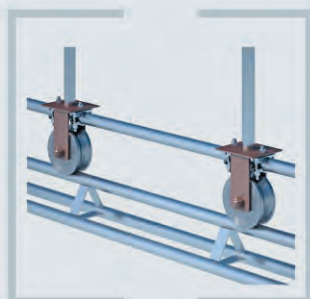
Flange/Guide roller 30 kN, Steel wheel Ø 200 mm Installation height 300 mm
